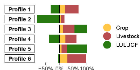
Figure 3: Composition of AFOLU emissions by profile
